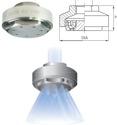
Spray section
